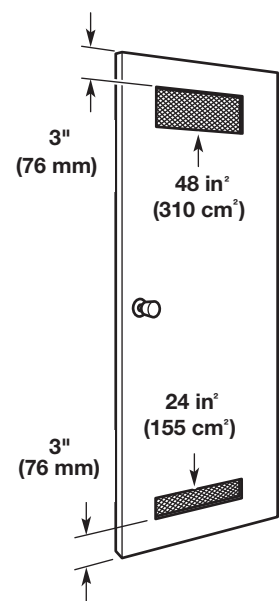
Closet Door Minimum Acceptable Vent Sizes
