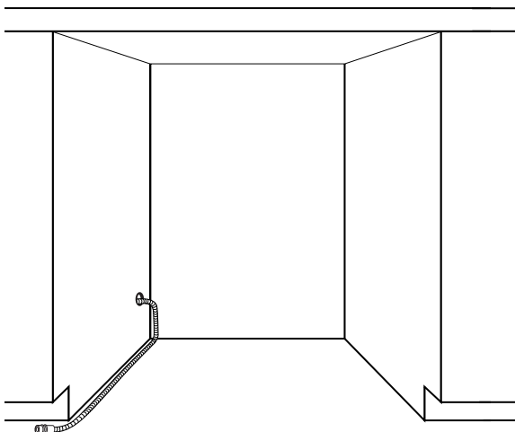
Route wire through 1 1/2" (3.81 cm) hole located 8" (20.32 cm) above the floor.
