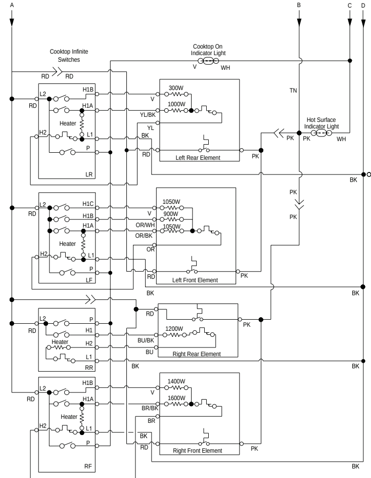
Cooktop Wiring Diagram
