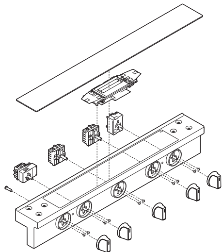
Front Control Console
