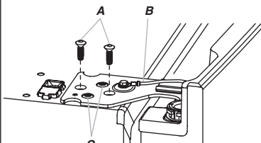
A. 3/16" Internal hex-head Screws B. Ground Wire (Do Not Remove) C. Screws (Do Not Remove)
