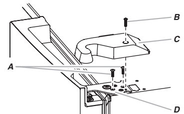
A. 3/16" Internal hex-head Screws B. Hinge Cover Screw C. Top Hinge Cover D. Top Hinge
