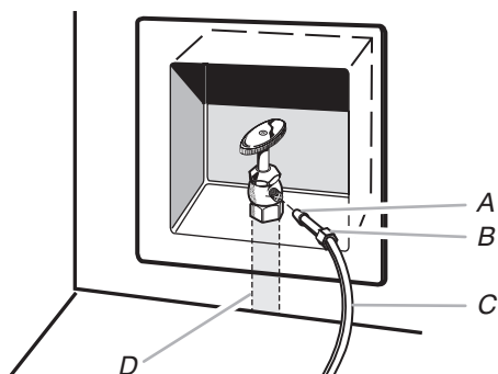
A. Sleeve B. Nut C. Copper tubing (to refrigerator) D. Household supply line \frac{1}{2} " (12.7 mm) minimum
