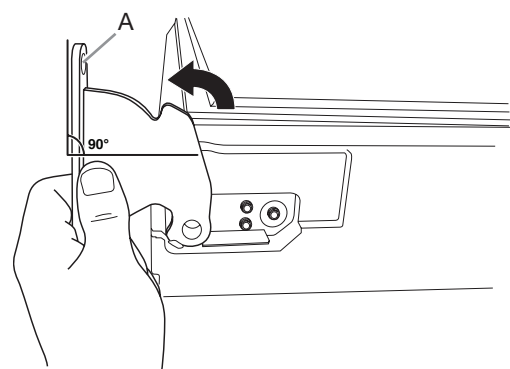
A. Hinge base turned to a 90° angle with the bottom edge of the door
