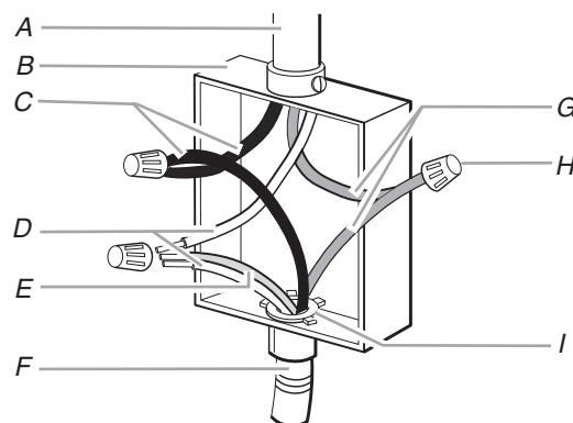
A. Cable from home power supply B. Junction box C. Black wires D. White wires E. Green (or bare) ground wire (from oven) F. 4-wire flexible cable from oven G. Red wires H. UL-listed wire connectors I. UL-listed or CSA-approved conduit connector
