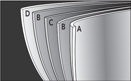
5-Layer Design: A. 18/10 Stainless Steel B. Aluminum C. Copper D. 18/0 Stainless Steel
