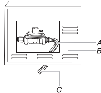
A. New CSA International approved “outdoor” flexible gas supply line B. Rear of grill C. To Natural gas supply
